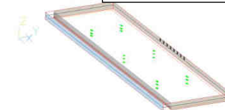
Iso-surface Ammonia @ 2nm
