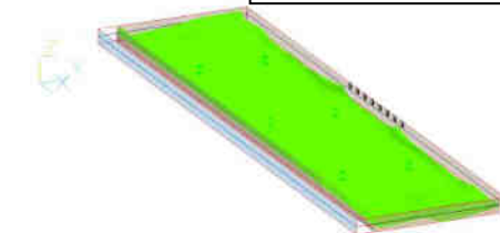
Iso-surface Ammonia @ 1ppm
