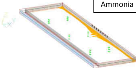
Iso-surface Ammonia @ 1.5ppm
