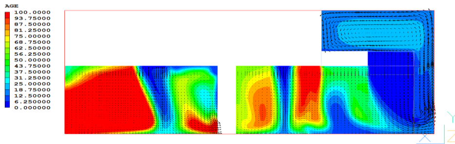
Figure 5 - Mean Age of Air Contours
