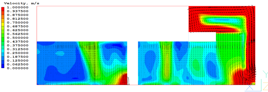
Figure 4 - Velocity Contours [vertical plane]
