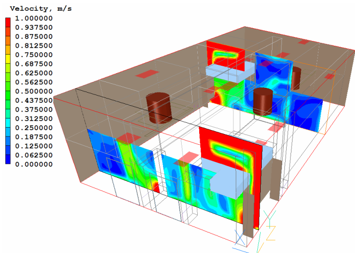
Figure 3 - air velocity @ vertical cross-section
