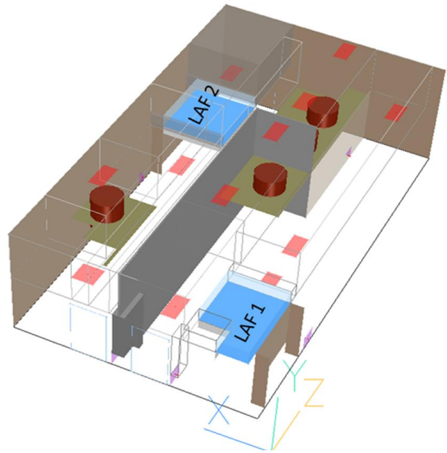
Figure 1 - Typical equipment layout in CFD model
