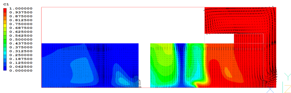
Figure 6 - Mass Fraction of LAF Air Contours
