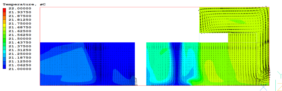
Figure 7 - Temperature Contours
