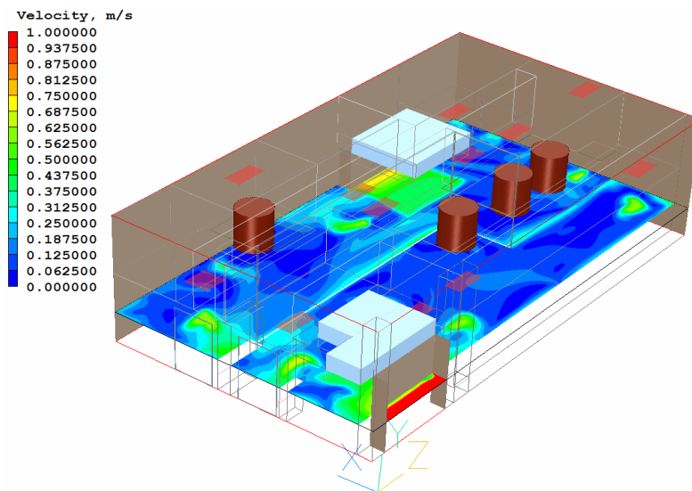
Figure 2 - air velocity @ 1.2m height
