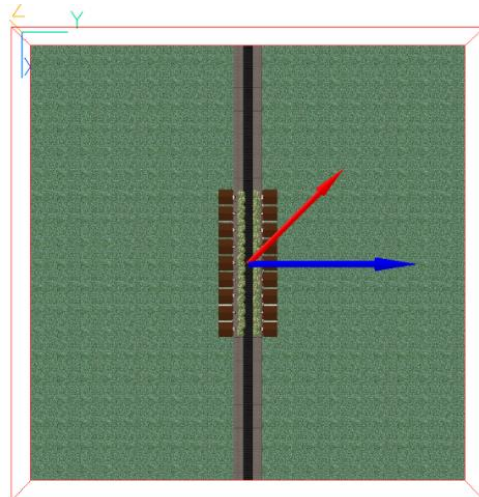
Figure 1: Street setup based on the model in Xue and Li (2017, Figure.1) [2]. Two rows of detached houses are separated by a central road and two rows of trees.
